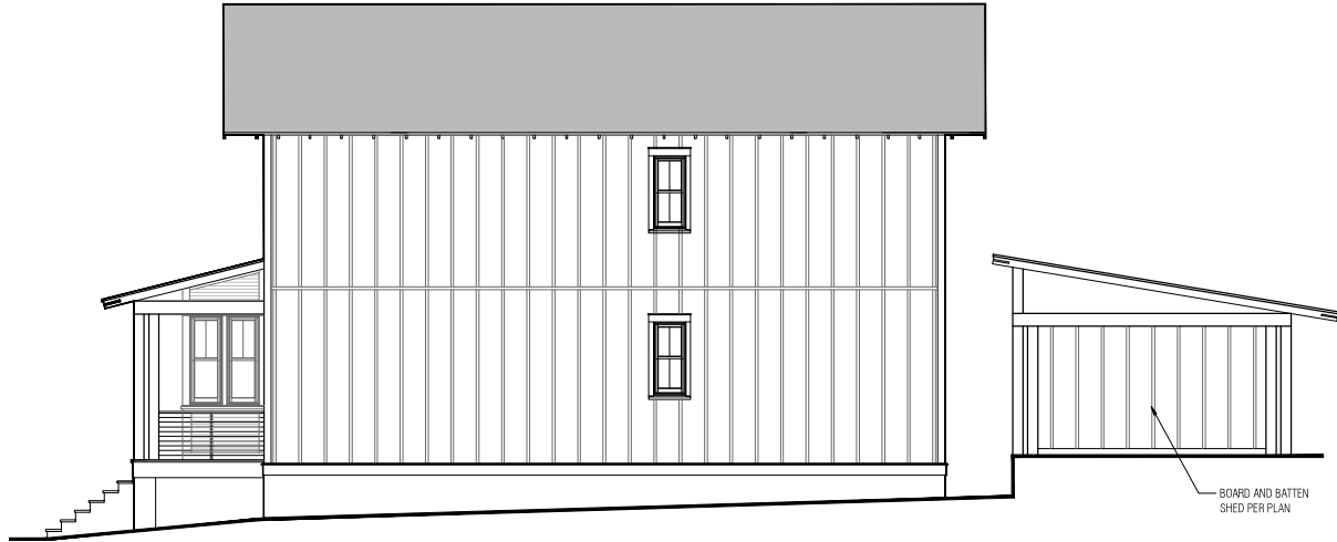
3 NORTH ELEVATION SCALE 1/4" = 1'
