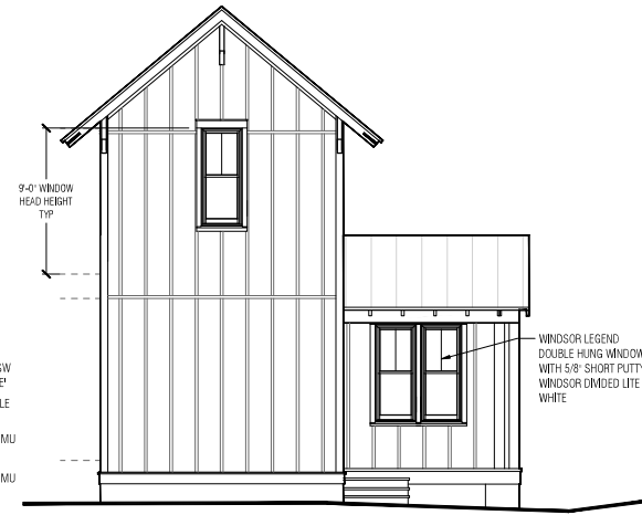
2 REAR ELEVATION SCALE 1/4" = 1'
