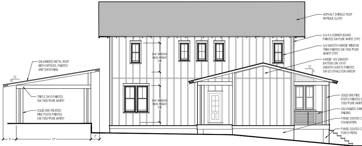
4 SOUTH ELEVATION SCALE 1/4" = 1'
