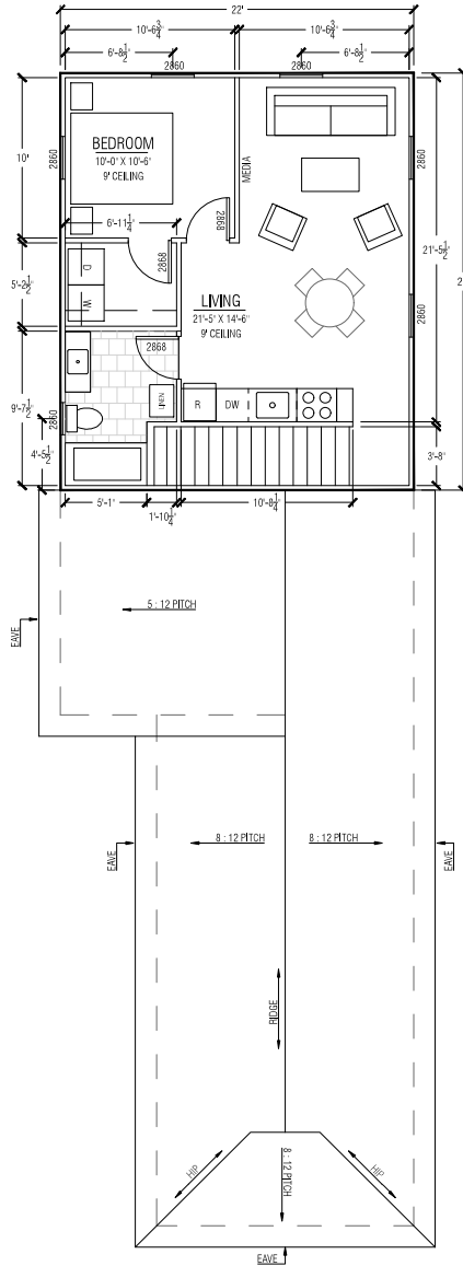
2 UPPER FLOOR SCALE 1/4" = 1'
