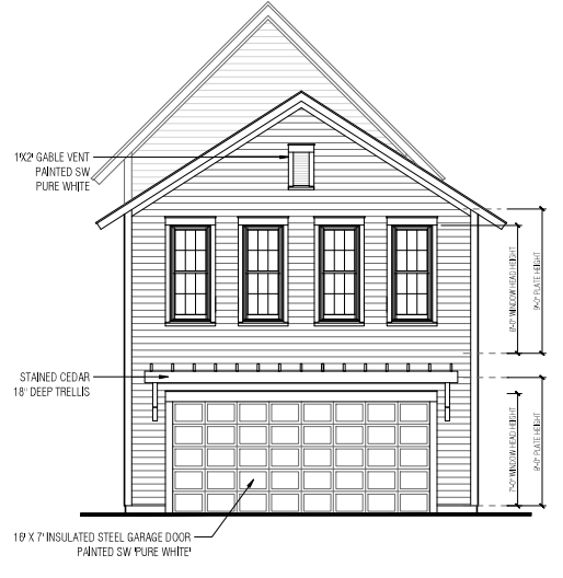
2 REAR ELEVATION SCALE 1/4" = 1'
