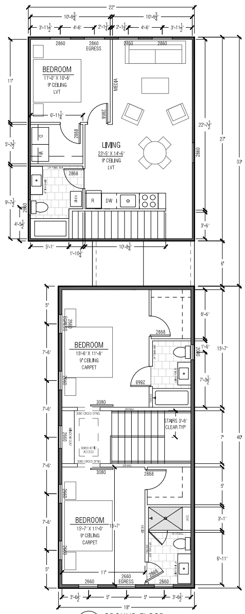
1 GROUND FLOOR SCALE 1/4" = 1'
