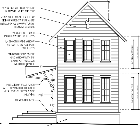
1 FRONT ELEVATION SCALE 1/4" = 1'
