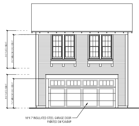
2 REAR ELEVATION SCALE 1/4" = 1'
