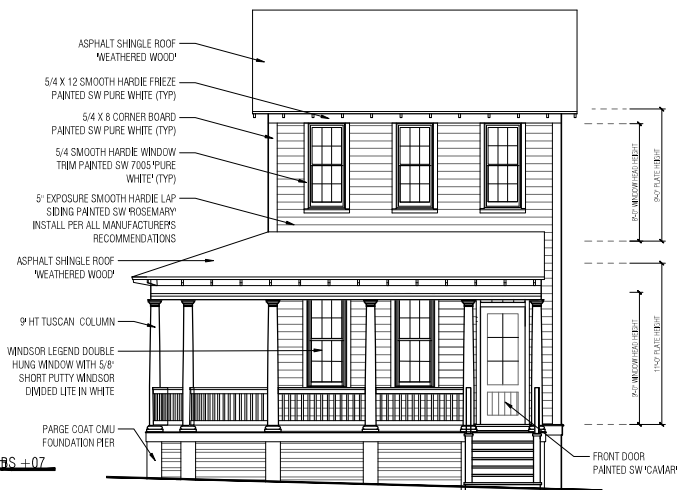
1 FRONT ELEVATION SCALE 1/4" = 1'
